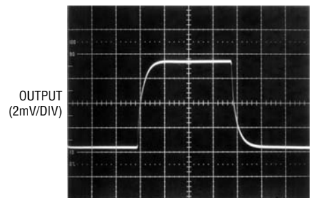
Large-Signal Transient Response ( I_S = 300\mu\text{A} per Amplifier)
