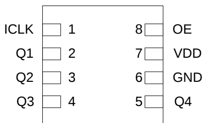
8-pin DFN
