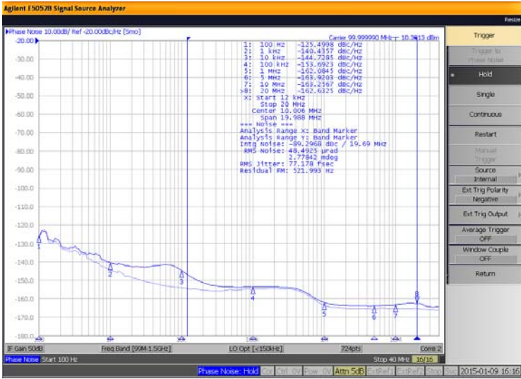
Figure 2. 651S Output Phase Noise 77fs (12kHz to 20MHz)
