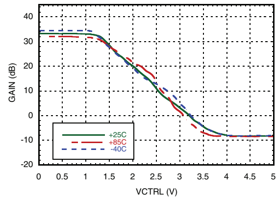
Gain vs. VCTRL @ 800MHz [2]
