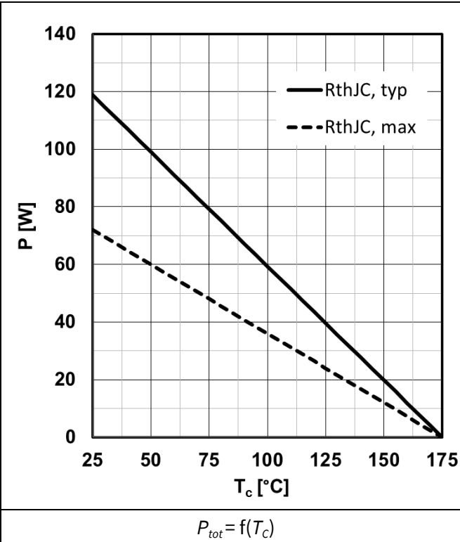
Figure 1 Power dissipation
