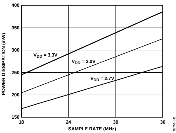
Figure 10. Power Curves
