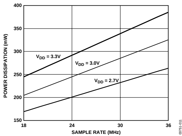
Figure 10. Power Curves
