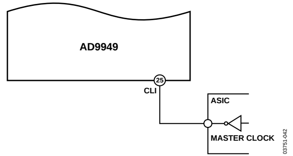
Figure 41. CLI Connection, DC-Coupled
