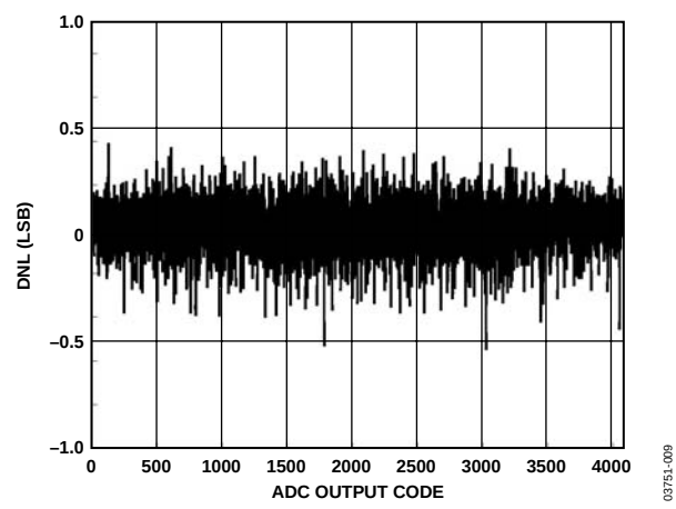
Figure 8. Typical DNL
