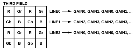
Figure 32. CCD Color Filter Example—Three-Field Readout
