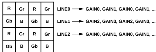
Figure 30. CCD Color Filter Example—Progressive Scan
