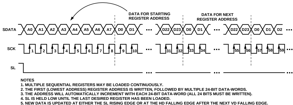
Figure 15. Continuous Serial Write Operation
