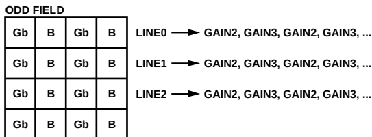
Figure 31. CCD Color Filter Example—Interlaced Readout
