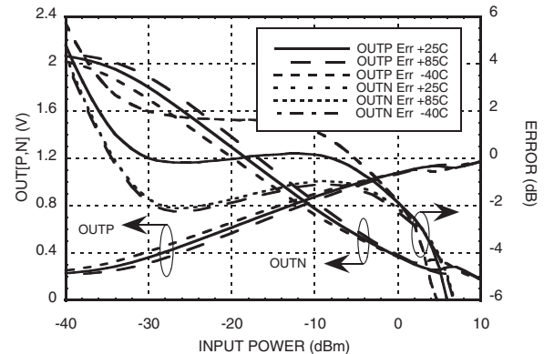
Output Voltage & Error vs. Input Power, F_{in} = 8000 MHz
