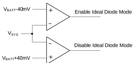
Figure 4: Ideal Diode Mode Enable/Disable
