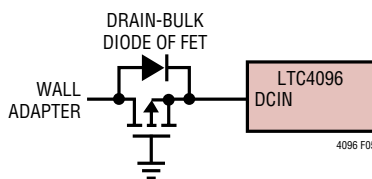
Figure 5. Low Loss Input Reverse Polarity Protection
