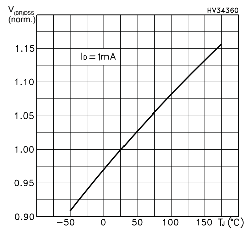
Figure 8. Normalized V_{(BR)DSS} vs temperature
