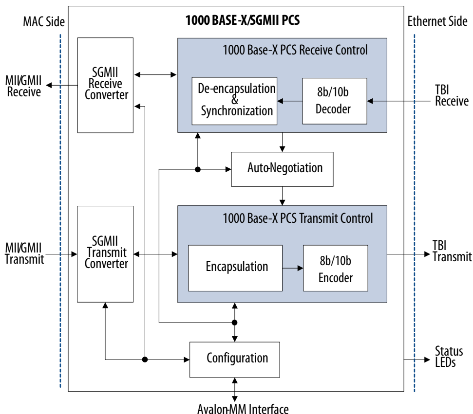
Figure 24. 1000BASE-X/SGMII PCS
