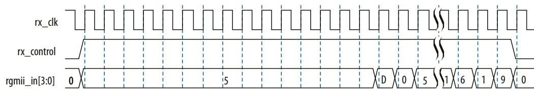
Figure 67. RGMII Receive in 1000 Mbps
