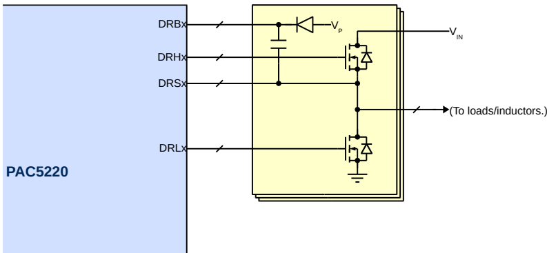
Figure 12-2 Typical Gate Driver Connections
