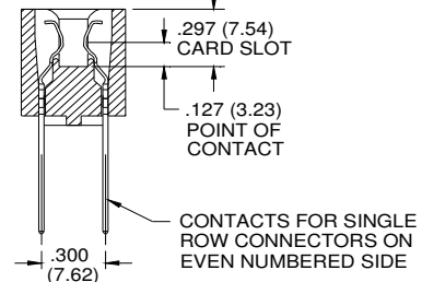
SECTION THROUGH CONTACT POSITION
