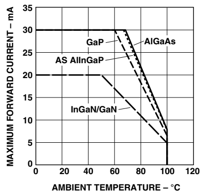
Figure 4b. Maximum forward current vs. ambient temperature. Derated based on T_{JMAX} = 110^{\circ}\text{C} , RO_{JA} = 700^{\circ}\text{C/W} (3 chip on)
