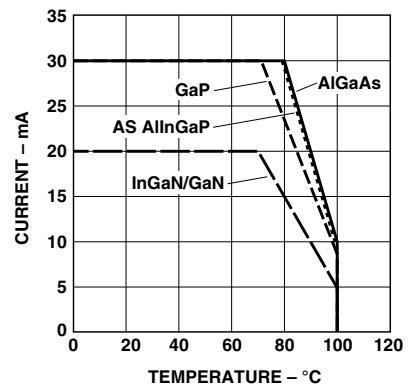
Figure 4a. Maximum forward current vs. ambient temperature. Derated based on T_{jMAX} = 110^{\circ}\text{C} , R_{\theta JA} = 500^{\circ}\text{C/W} (1 chip on)
