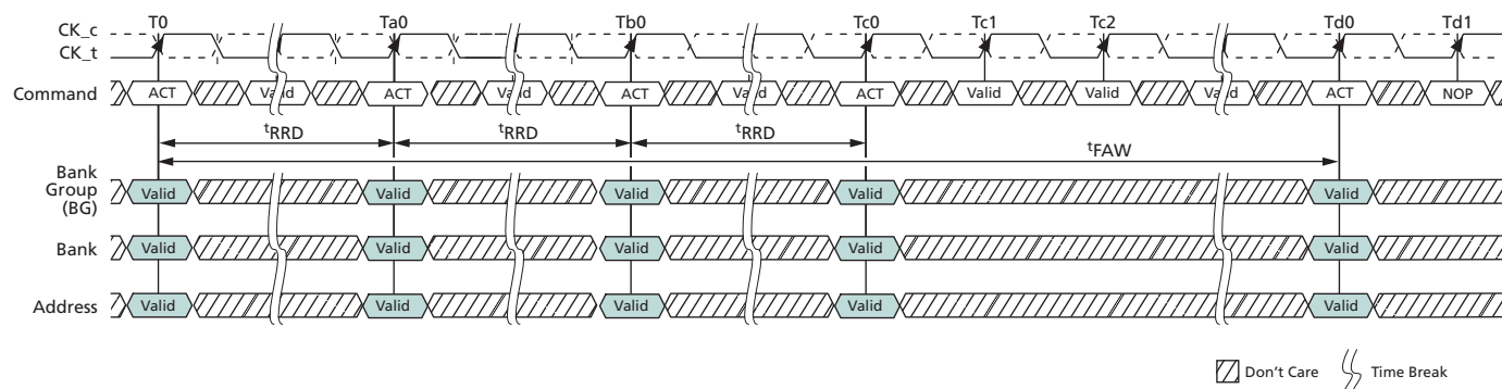
Figure 82: t_{FAW} Timing
