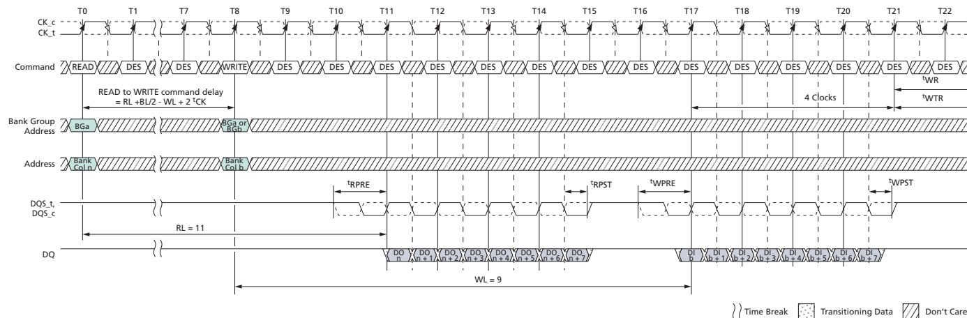
Figure 142: READ (BL8) to WRITE (BL8) with 1 st CK Preamble in Same or Different Bank Group
