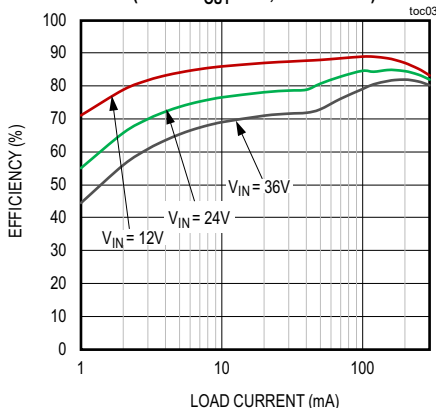
EFFICIENCY vs. LOAD CURRENT (FIXED V_{OUT} = 5V , PFM MODE)
