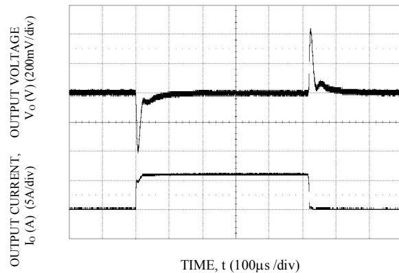
Transient Response to Dynamic Load Change from 0% to 50% to 0%. V_o=2.5V
