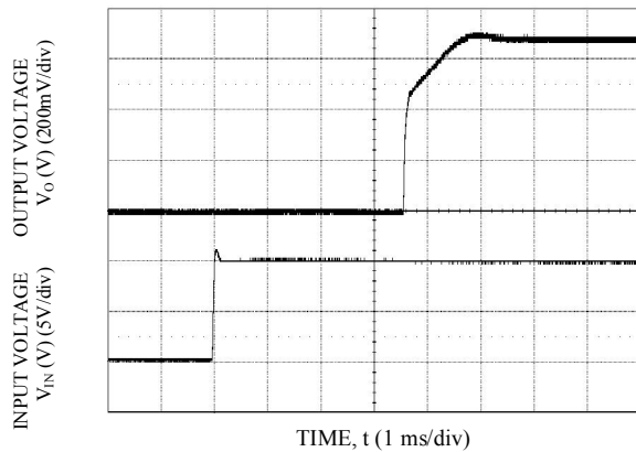
Start-up Using Input Voltage ( V_{IN} = 10V , I_o = I_{o,max} ), V_o = 0.69V
