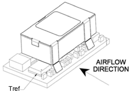
Preferred airflow direction and location of hot-spot of the module ( T_{ref} ).
