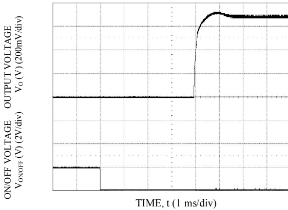
Start-up Using On/Off Voltage ( I_o = I_{o,max} ), V_o=0.69V
