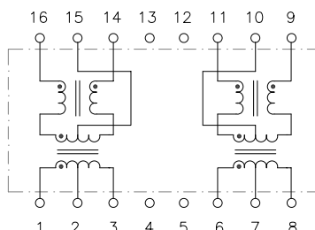
Circuit D
