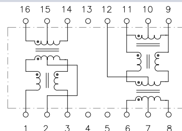
N6 Package
