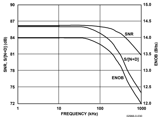
Figure 10. SNR, S/[\text{N}+\text{D}] , and ENOB vs. Frequency
