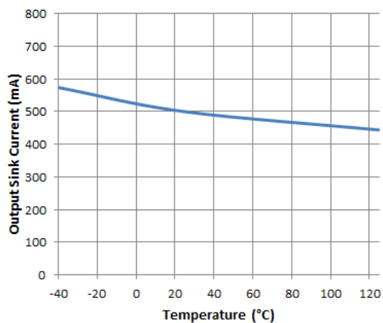
Figure 16. Output Sink Current vs. Temperature
