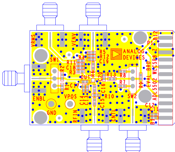
Figure 66. Layout of Evaluation Board, Component Side
