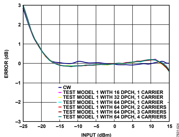
Figure 24. Error from CW Linear Reference vs. Input with Various W-CDMA Forward Link Waveforms at 2200 MHz, C_{FLT} = 10 nF, C_{OUT} = \text{Open}
