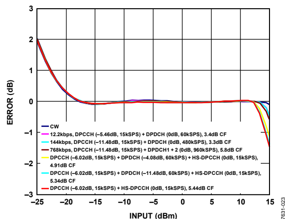
Figure 23. Error from CW Linear Reference vs. Input with Various W-CDMA Reverse Link Waveforms at 900 MHz, C_{FLT} = 10 nF, C_{OUT} = \text{Open}
