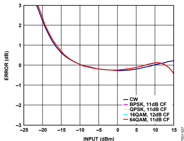
Figure 27. Error from CW Linear Reference vs. Input with Various 802.16 OFDM Waveforms at 3500 MHz, 10 MHz Signal BW, and 256 Subcarriers for All Modulated Signals, C_{FLT} = 10 nF, C_{OUT} = \text{Open}
