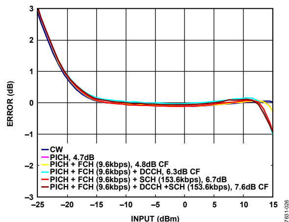
Figure 26. Error from CW Linear Reference vs. Input with Various CDMA2000 Reverse Link Waveforms at 1900 MHz, C_{FLT} = 10 nF, C_{OUT} = \text{Open}
