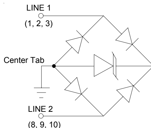
Circuit Diagram
