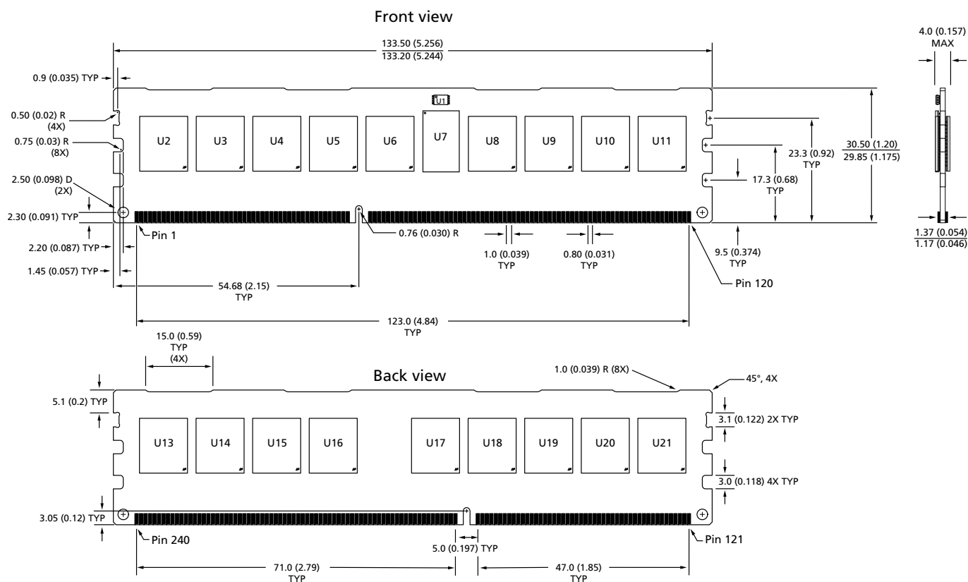
Figure 4: 240-Pin DDR3 RDIMM R/C B1 (PCB 1164)
