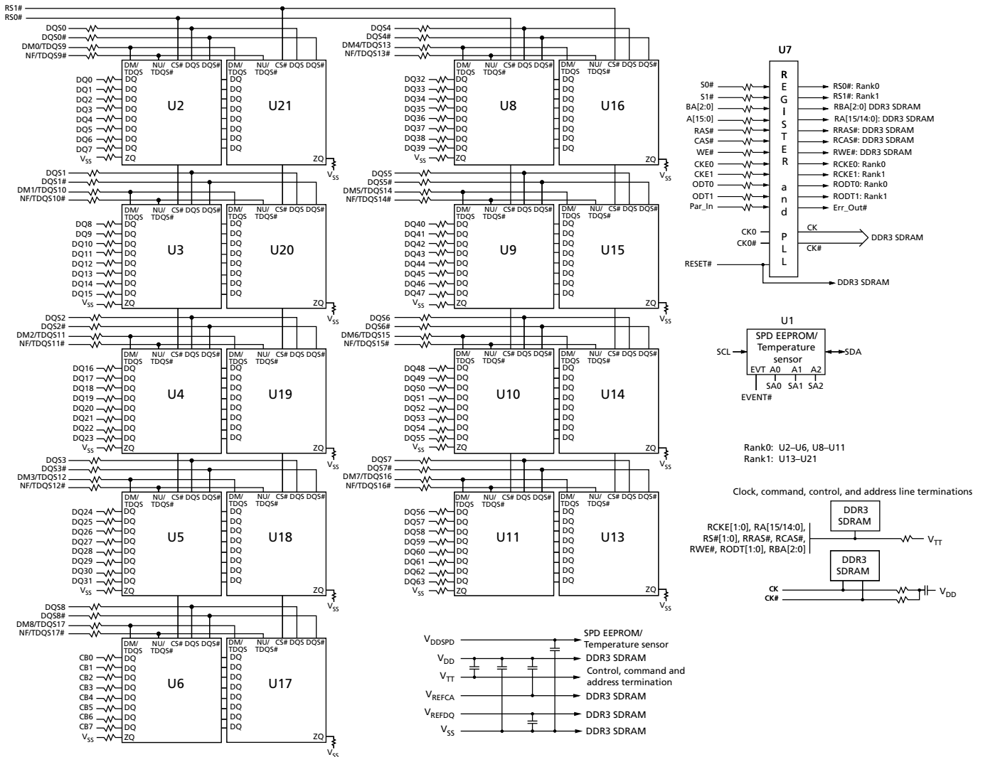
Figure 3: Functional Block Diagram R/C B1(PCB 1164 and 1560)
