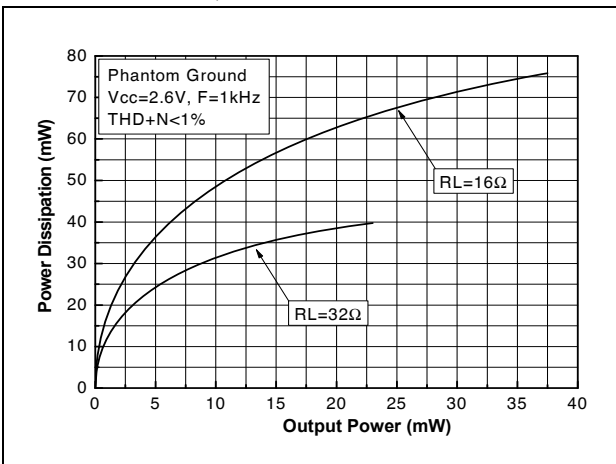
Figure 42. Power dissipation vs. output power, PHG, V_{CC} = 2.6\text{ V}
