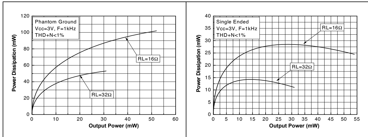
Figure 44. Power dissipation vs. output power, PHG, V_{CC} = 3\text{ V} Figure 45. Power dissipation vs. output power, SE, V_{CC} = 3\text{ V}
