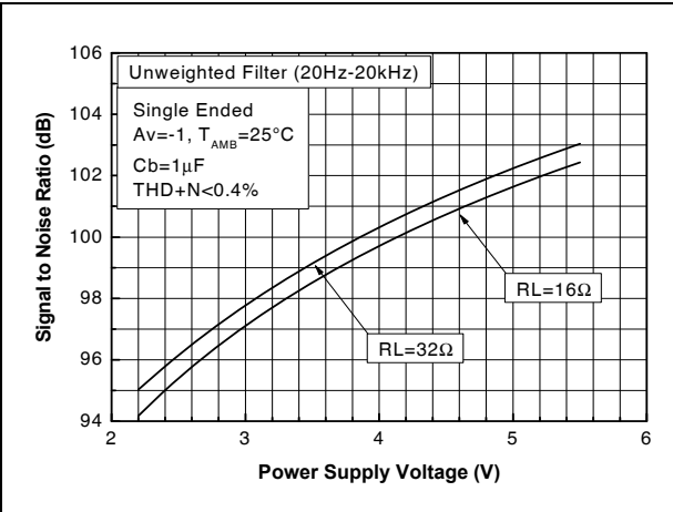
Figure 55. SNR vs. power supply voltage, SE, unweighted, A_v = 1
