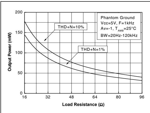
Figure 40. Output power vs. load resistance, PHG, V_{CC} = 5\text{ V}
