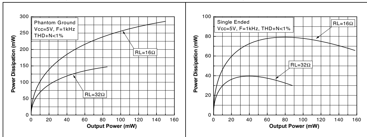
Figure 46. Power dissipation vs. output power, PHG, V_{CC} = 5\text{ V} Figure 47. Power dissipation vs. output power, SE, V_{CC} = 5\text{ V}
