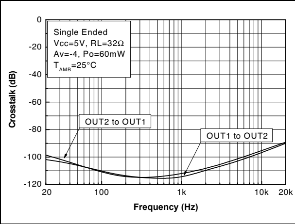
Figure 53. Crosstalk vs. frequency, PHG, V_{CC} = 5\text{ V} , A_v = 4
