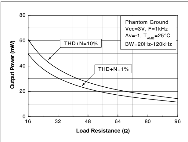
Figure 38. Output power vs. load resistance, PHG, V_{CC} = 3\text{ V}
