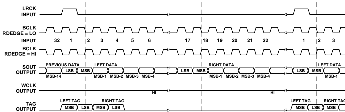
Figure 16. Serial Data Output Timing: Slave Mode, I^2S -Justified, 32-Bit Frame Mode, \overline{S}M = HI , RLJUST = LO , \overline{MSBDLY} = LO
