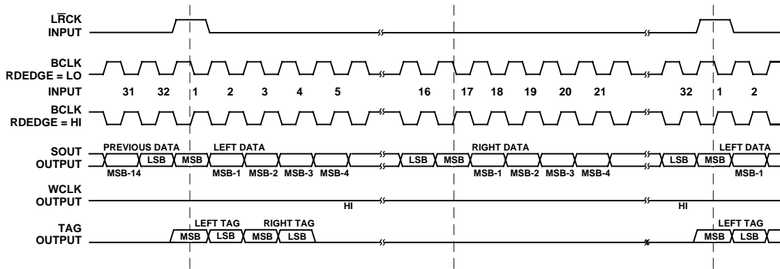
Figure 15. Serial Data Output Timing: Slave Mode, Left-Justified with No MSB Delay, 32-Bit Frame Mode, \overline{S}M = HI , RLJUST = LO , \overline{MSBDLY} = HI
