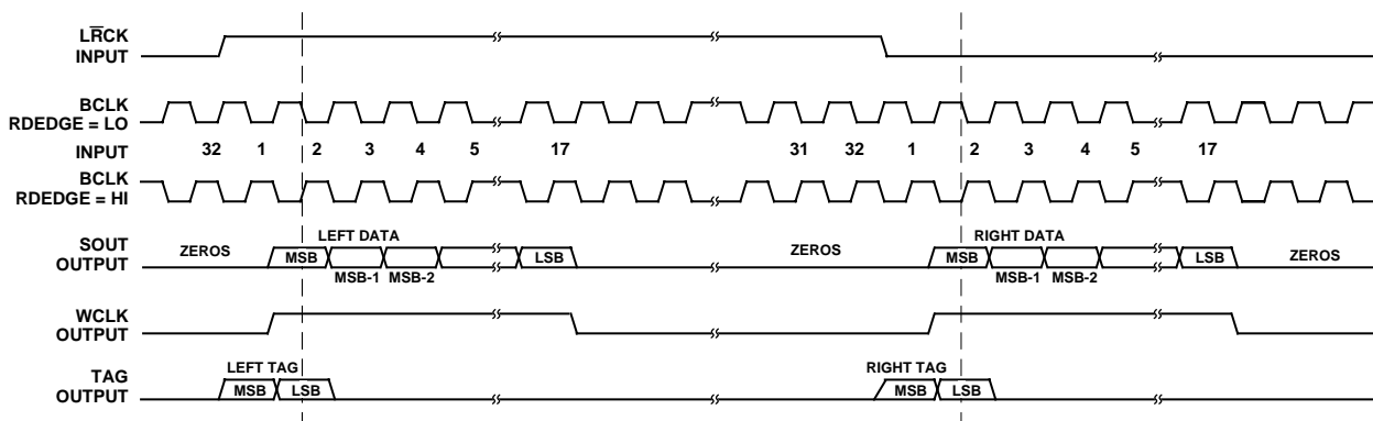
Figure 10. Serial Data Output Timing: Slave Mode, P \hat{S} -Justified, S\overline{M} = HI , RLJUST = LO , MSBDLY = LO
