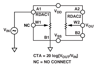
Figure 38. Analog Crosstalk
