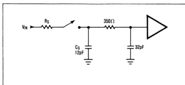
Figure 8. Equivalent Input Model
