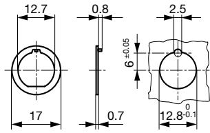
Transparent Cover 0853.0551 Reflow-Cover 0853.0571 Order No. _____ OGN/OGN-SMD 0853.0551 * / 0853.0571 *
