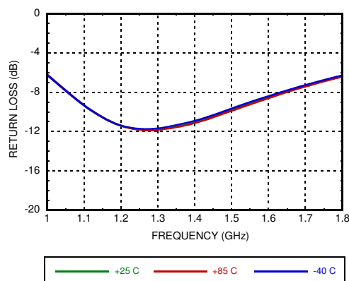
Output Return Loss vs. Temperature [1]
