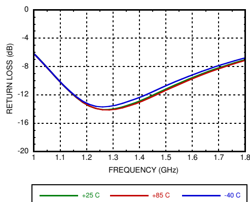
Output Return Loss vs. Temperature [2]
