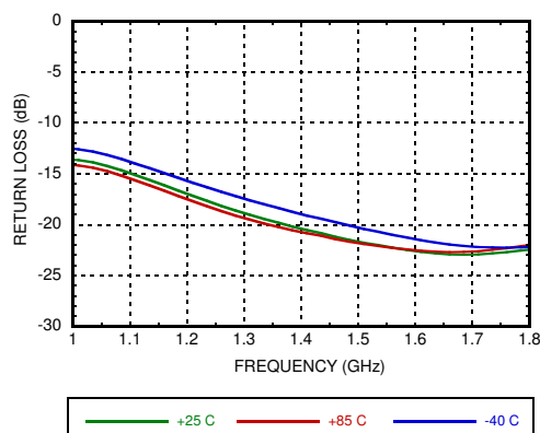
Input Return Loss vs. Temperature [2]
