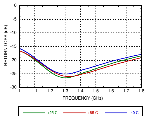
Input Return Loss vs. Temperature [1]
