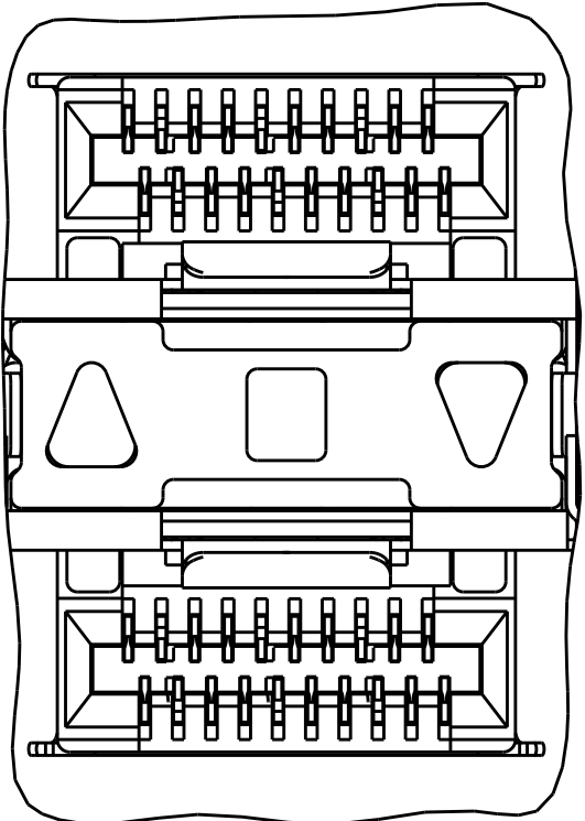
CENTER/REVERSED OUTER LIGHT PIPES 1-2198318-7, 1-2198318-9 SCALE 5:1
