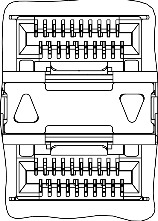
REVERSED OUTER LIGHT PIPES 1-2198318-8, 2-2198318-0 SCALE 5:1
