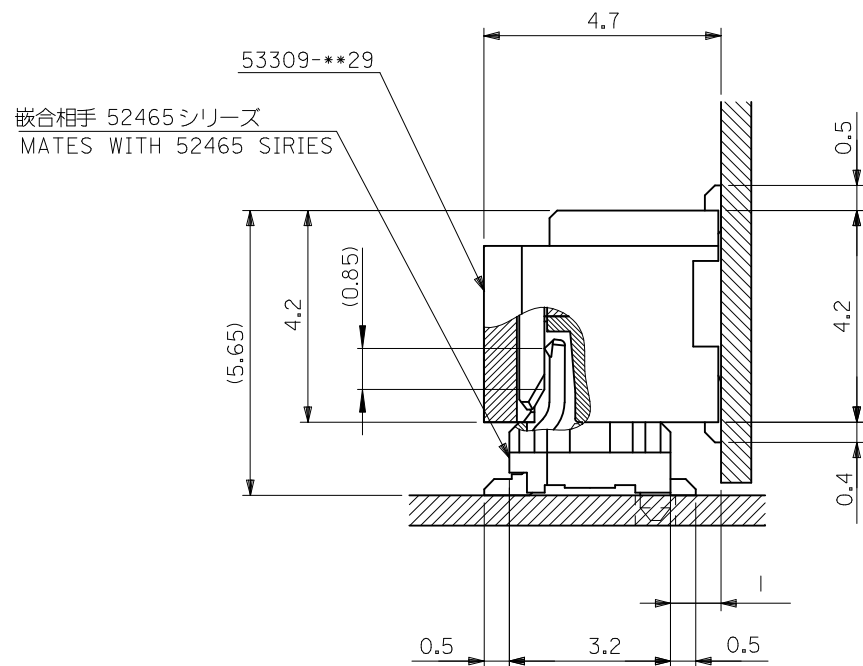
嵌合状態図 (参考) MATED DRAWING(REF.)
