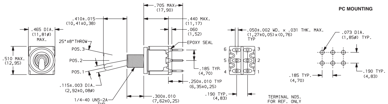
DPDT
