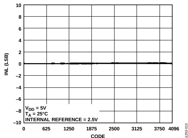
Figure 11. Integral Nonlinearity (INL) vs. Code
