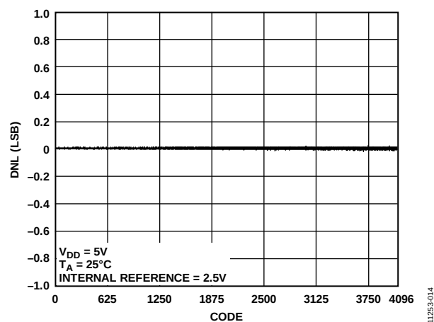
Figure 12. Differential Nonlinearity (DNL) vs. Code
