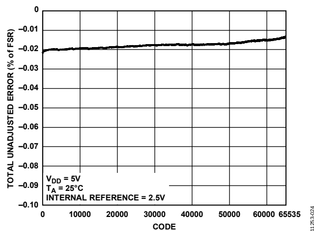
Figure 22. Total Unadjusted Error vs. Code
