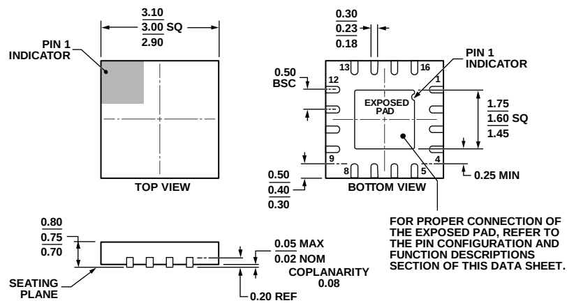
Figure 53. 16-Lead Lead Frame Chip Scale Package [LFCSP_WQ] 3 mm × 3 mm Body, Very Very Thin Quad (CP-16-22)
