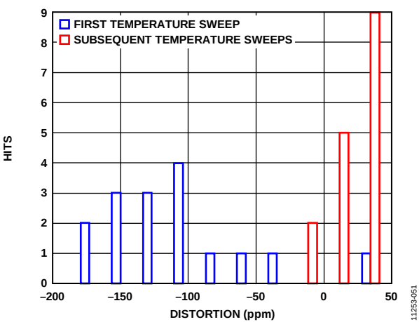
Figure 49. Thermal Hysteresis
