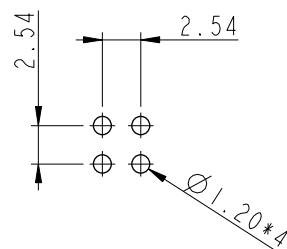
4 Pin Male Connector Male Pin PCB Layout
