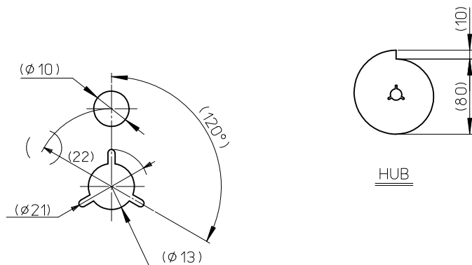
DETAIL "F"
