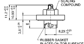
Shellsize 1-4
