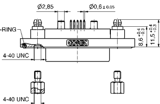
Shellsize 1-4
