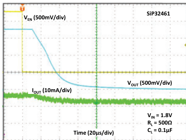
Fig. 41 - Turn-off Time
