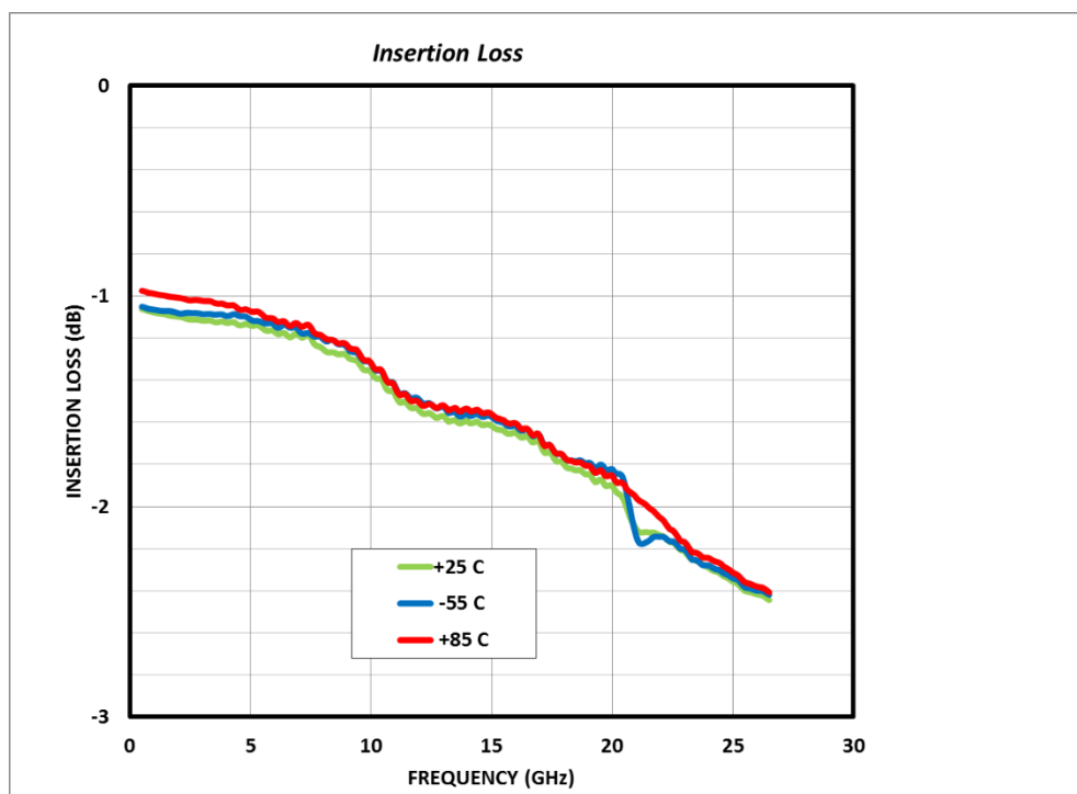
Figure 2 Insertion Loss vs. Temperature
