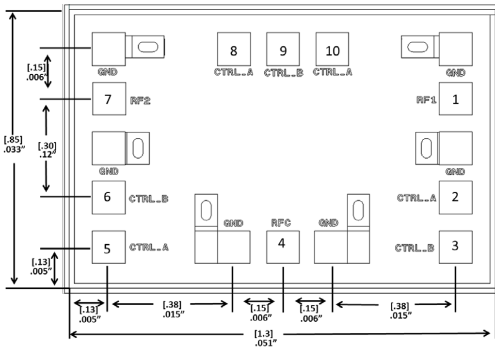
Figure 7 Chip Outline
