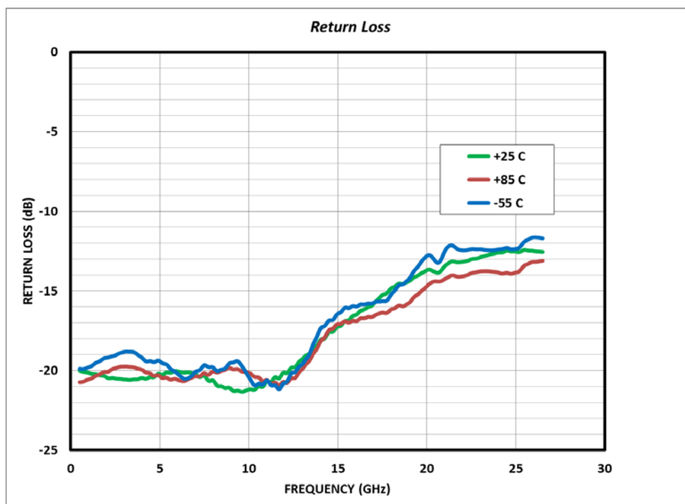
Figure 4 Return Loss vs. Temperature
