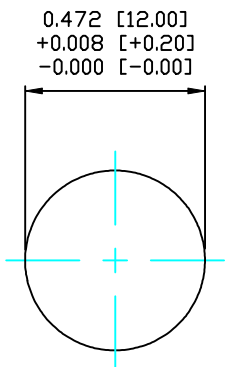
PANEL CUTOUT
