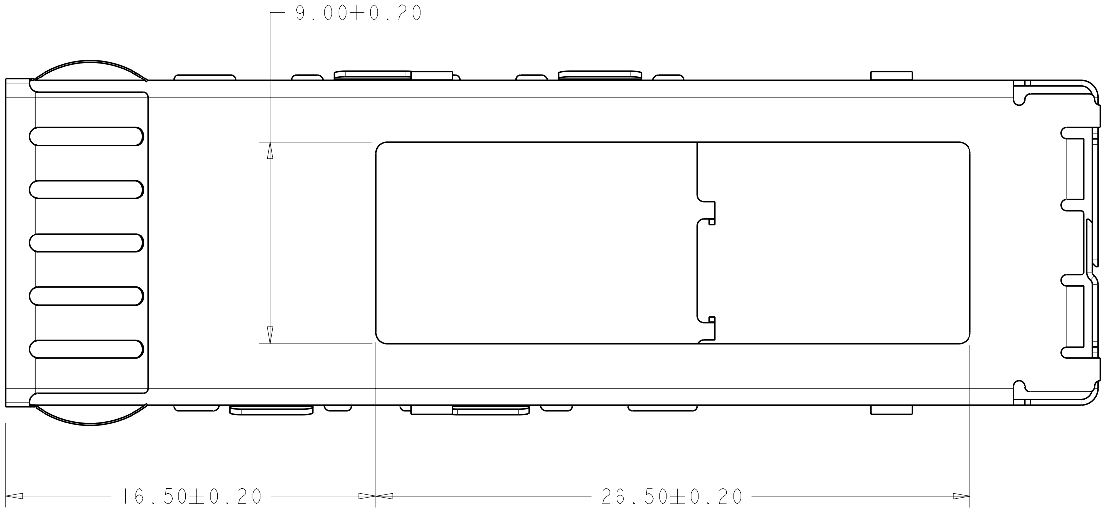
2007198-2 SAME AS 2007198-1 EXCEPT AS SHOWN TOP VIEW
