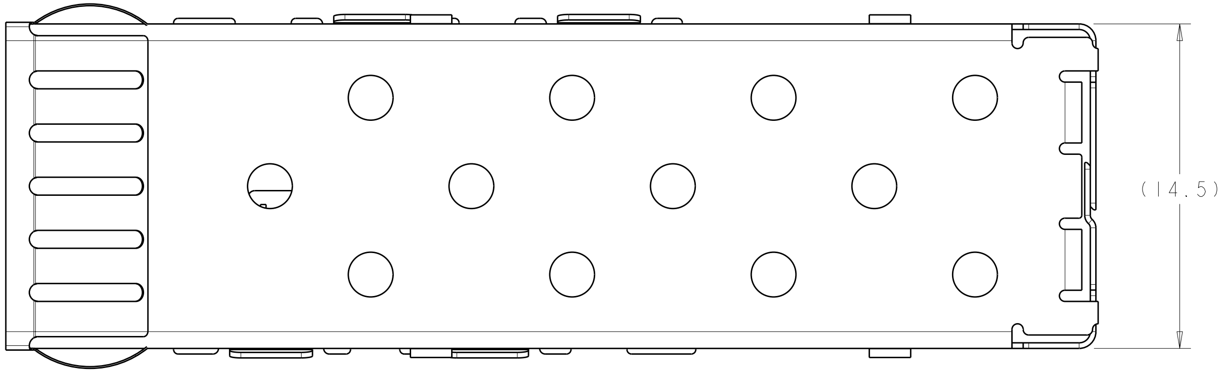
2007198-1 TOP VIEW
