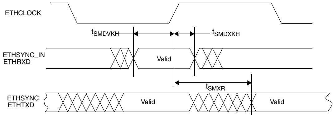
Figure 18. SMII Mode Signal Timing
