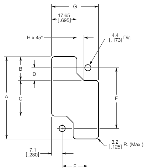
Recommended Panel Cutout for Receptacles (Pin Housings)
