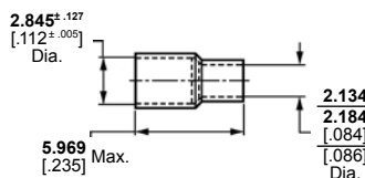
Ferrule Part No. 1-332057-0
