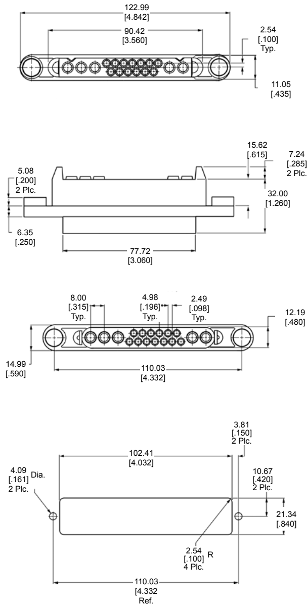
Recommended Panel Cutout
