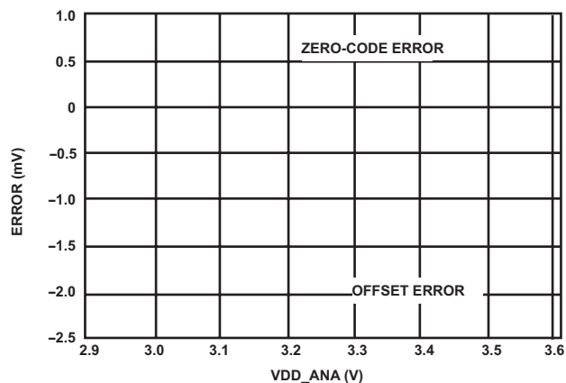
Figure 27. Zero-Code Error and Offset Error vs. Supply
