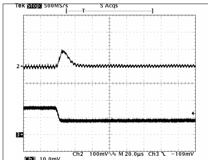
Fig 2.0V-7: Output voltage response for V_{out}=2.0V to negative load current step change from 8A to 4A with slew rate of -5A/\mu s at V_{in}=12V . C_o=47\mu F \times 2 ceramic. Top trace: output voltage (100mV/div.) Bottom trace: load current (2A/div.) Time scale: 20\mu s /div.
