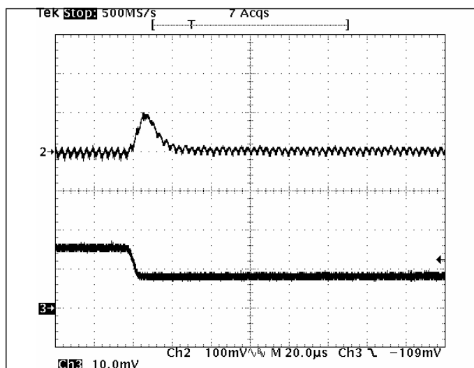
Fig 2.5V-7: Output voltage response for V_{out}=2.5V to negative load current step change from 8A to 4A with slew rate of -5A/\mu s at V_{in}=12V . C_o=47\mu F \times 2 ceramic. Top trace: output voltage (100mV/div.) Bottom trace: load current (2A/div.) Time scale: 20\mu s /div.
