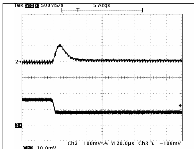
Fig 1.2V-7: Output voltage response for V_{out}=1.2V to negative load current step change from 8A to 4A with slew rate of -5A/\mu s at V_{in}=12V . C_o=47\mu F \times 2 ceramic. Top trace: output voltage (100mV/div.) Bottom trace: load current (2A/div.) Time scale: 20\mu s /div.
