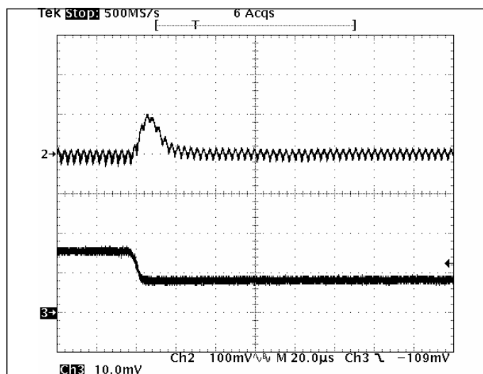
Fig 3.3V-7: Output voltage response for V_{out}=3.3V to negative load current step change from 8A to 4A with slew rate of -5A/\mu s at V_{in}=12V . C_o=47\mu F \times 2 ceramic. Top trace: output voltage (100mV/div.) Bottom trace: load current (2A/div.) Time scale: 20\mu s /div.
