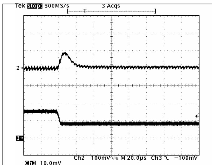
Fig 1.5V-7: Output voltage response for V_{out}=1.5V to negative load current step change from 8A to 4A with slew rate of -5A/\mu s at V_{in}=12V . C_o=47\mu F \times 2 ceramic. Top trace: output voltage (100mV/div.) Bottom trace: load current (2A/div.) Time scale: 20\mu s /div.
