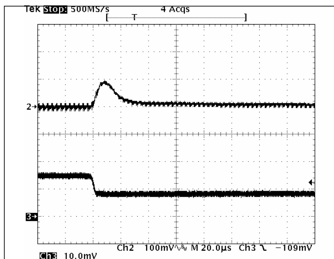
Fig 1.0V-7: Output voltage response for V_{out}=1.0V to negative load current step change from 8A to 4A with slew rate of -5A/\mu s at V_{in}=12V . C_o=47\mu F \times 2 ceramic. Top trace: output voltage (100mV/div.) Bottom trace: load current (2A/div.) Time scale: 20\mu s /div.
