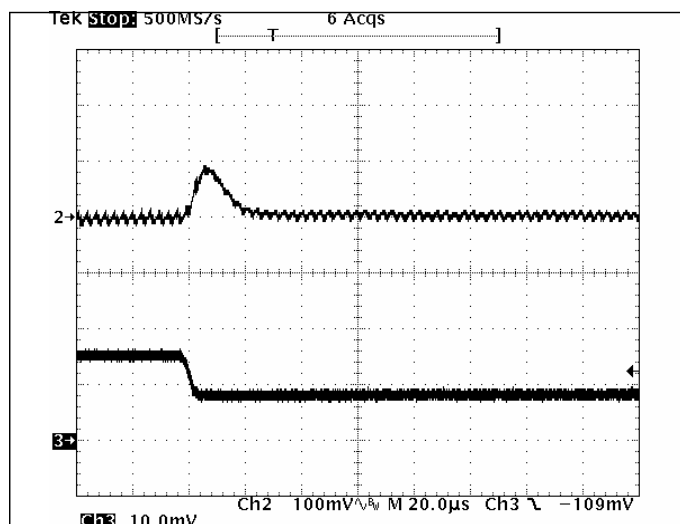
Fig 1.8V-7: Output voltage response for V_{out}=1.8V to negative load current step change from 8A to 4A with slew rate of -5A/\mu s at V_{in}=12V . C_o=47\mu F \times 2 ceramic. Top trace: output voltage (100mV/div.) Bottom trace: load current (2A/div.) Time scale: 20\mu s /div.
