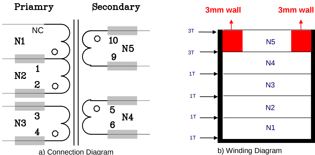
Figure 13: Transformer Structure
